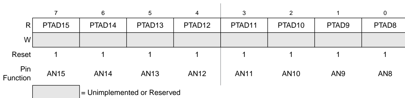
Figure 4-16. Port Data Register 0 (PORTAD0)
