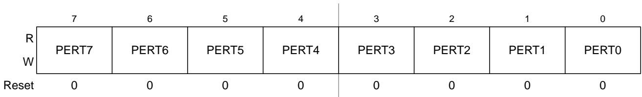
Figure 23-23. Port T Pull Device Enable Register (PERT)
