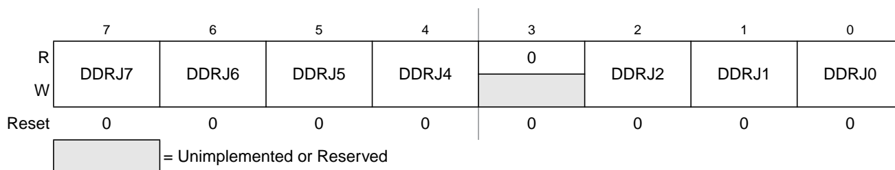
Figure 22-58. Port J Data Direction Register (DDRJ)
