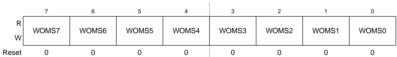
Figure 23-31. Port S Wired-OR Mode Register (WOMS)
