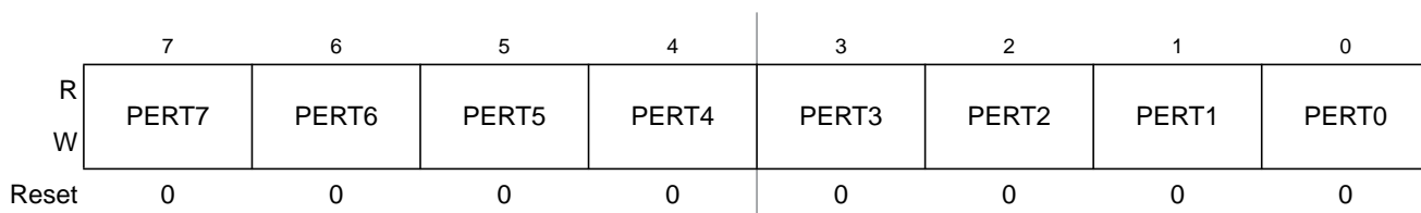
Figure 24-19. Port T Pull Device Enable Register (PERT)
