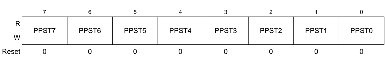
Figure 23-24. Port T Polarity Select Register (PPST)
