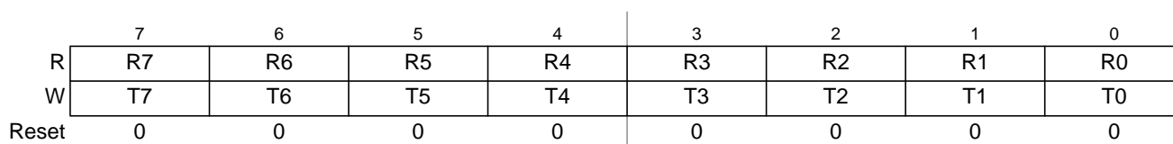
Figure 11-13. SCI Data Registers (SCIDRL)
